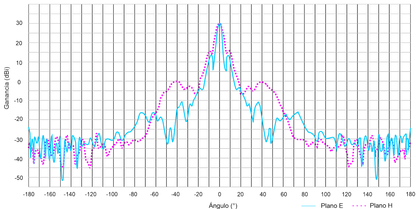
Antena NetPoint NP62 (NP6-DP-2FT)
